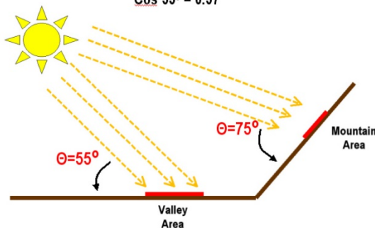
Figure 11: Insolation of angled ground
