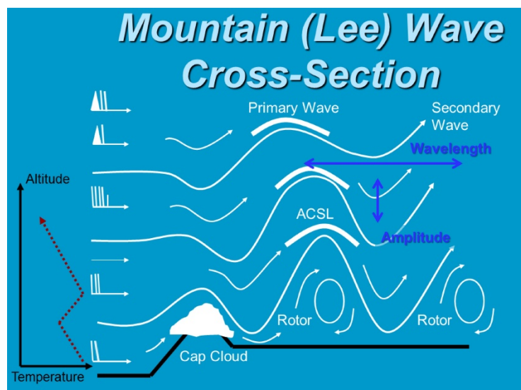
Figure 40: Mountain Wave Conceptual Model
