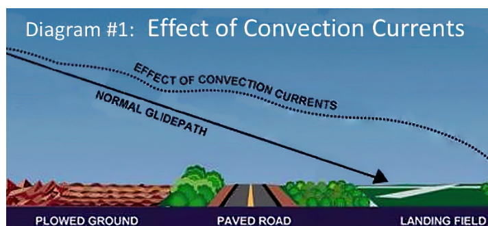
Figure 76: Glidepath Altered by Thermals
