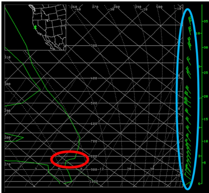
Figure 37: Classic Mountain Lee Wave Upper-Air Sounding March 16, 2001
