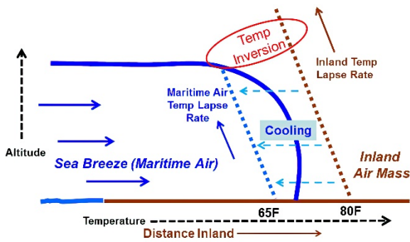
Figure 53: Sea Breeze Vertical Temperature Profile
