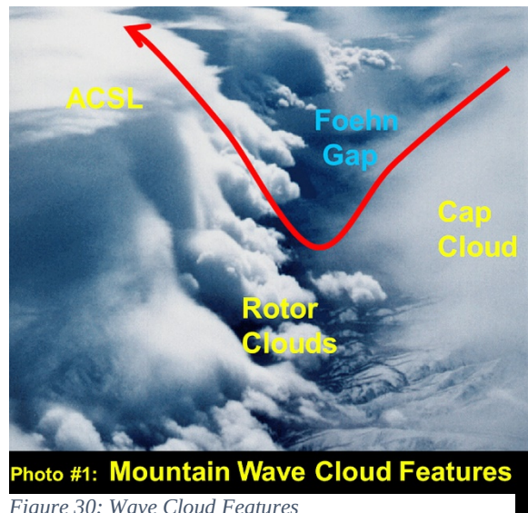
Photo #1: Mountain Wave Cloud Features
