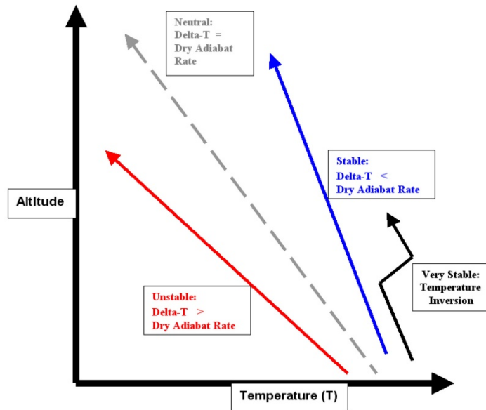
Figure 16 Atmospheric Instability Relative to Lapse Rates:
