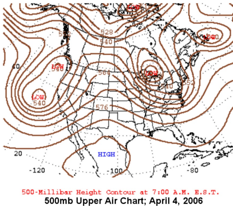
Figure 6: Upper-Air Synoptic Chart
