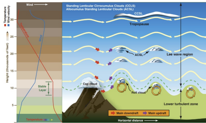
Figure 9-25. Mountain lee wave system.
