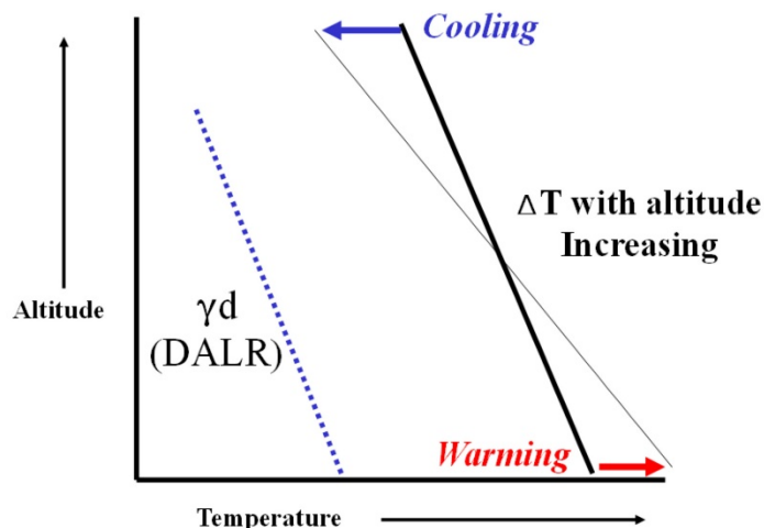
Figure 21: Destabilizing factors: temperature
