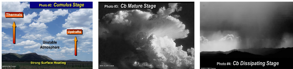
Figure 82: The 3 Thunderstorm Stages
