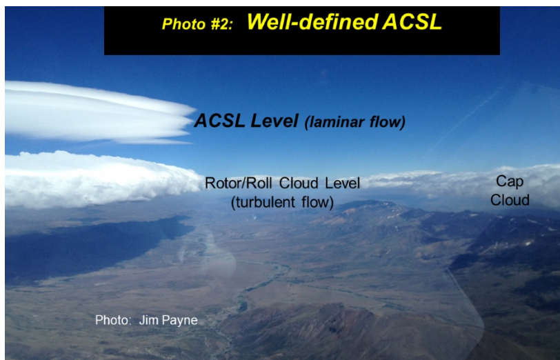
Figure 31: Well-defined ACSL
