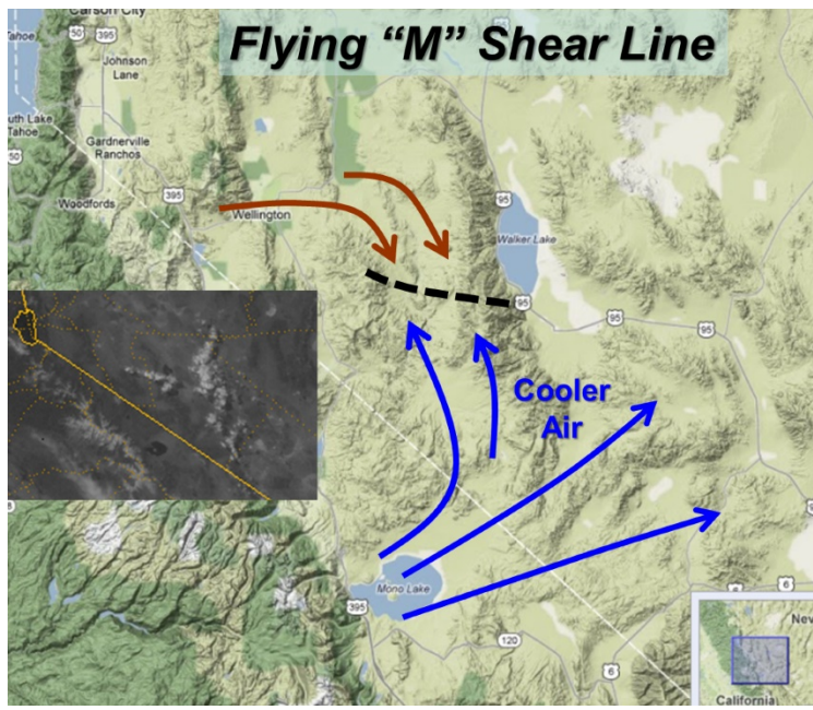
Figure 62: Flying M Shear Line
