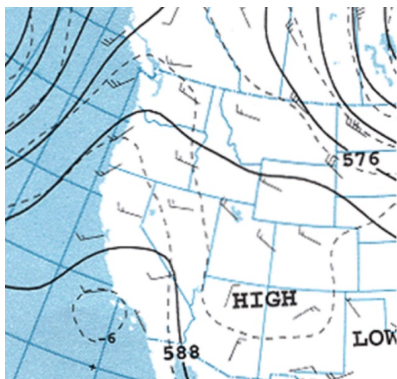
500 Mb Upper Air Chart June 14, 1999
