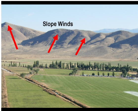
Figure 13: Terrain with Moderate Slope Wind
