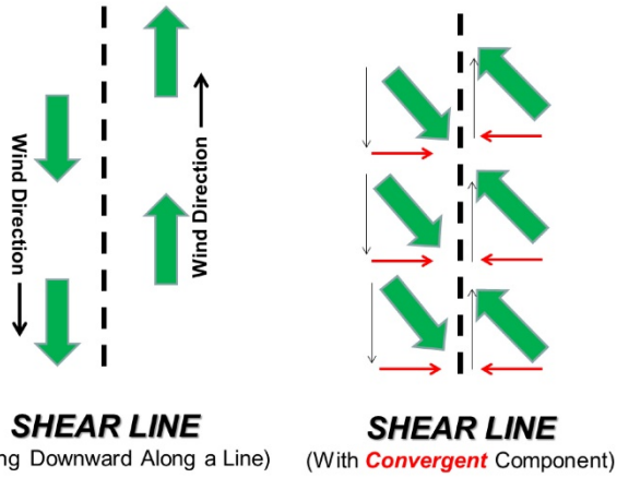
Figure 47: Shear Lines
