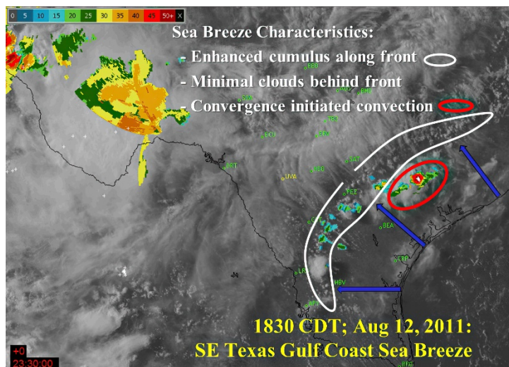
Figure 55: Deep Convection with Sea Breeze
