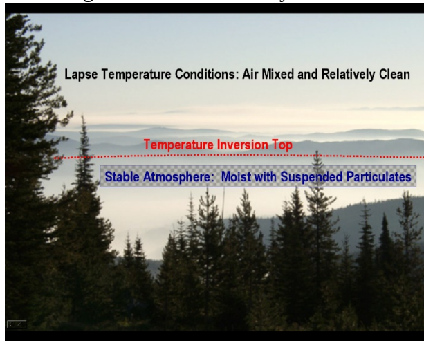
Figure 12: Valley Inversion, with Fog
