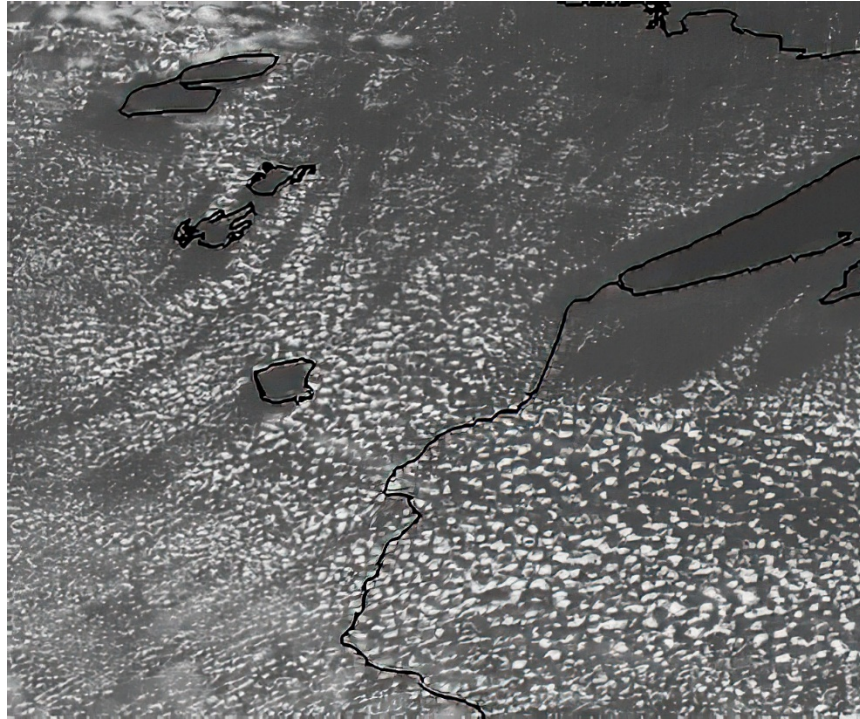
Figure 94: NE MN NW WI - Effect of water on thermal development.
