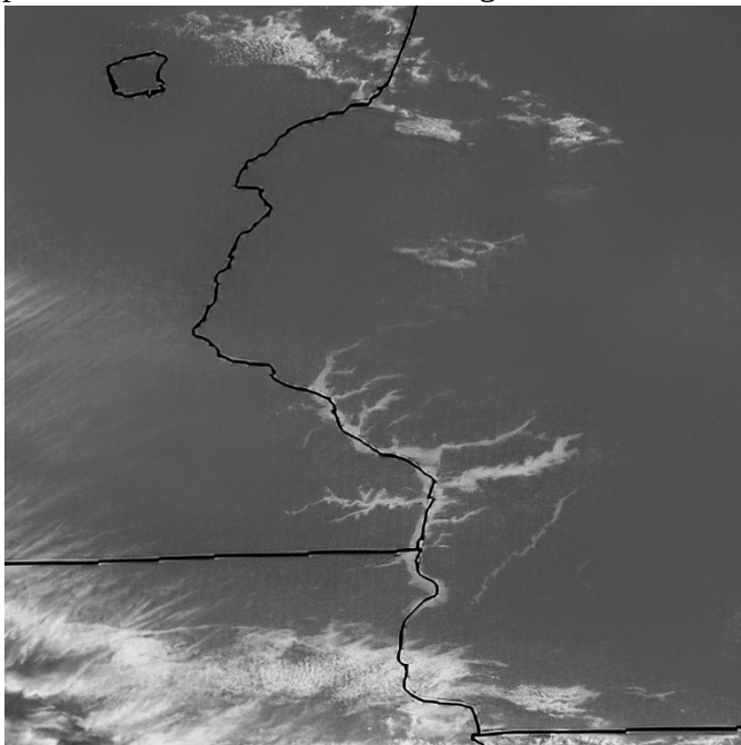
Figure 87: Early-morning radiation fog, MN-WI Mississippi & tributaries
