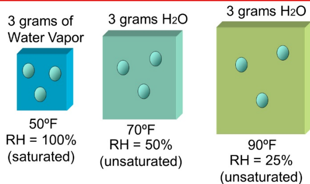
Figure 23: The Principle of Relative Humidity
