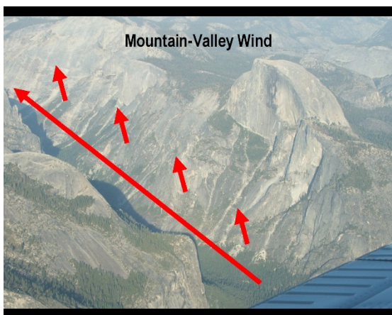
Figure 15: Terrain and Wind May Create Hazard
