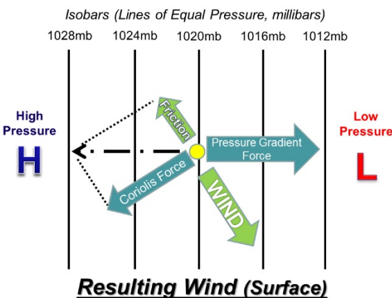
Figure 43: Coriolis Effect
