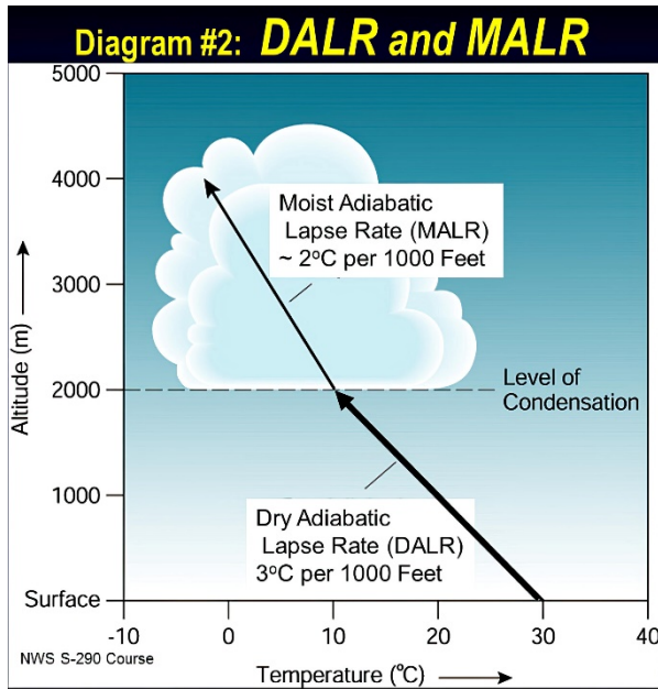
Figure 84: Lapse Rates, dry v moist
