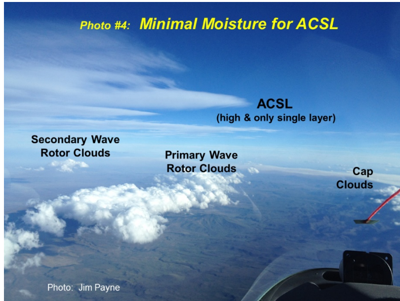
Figure 33: Minimal-Moisture ACSL
