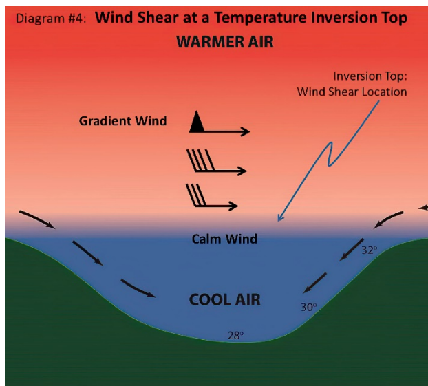
Figure 79: Wind Shear Above a Nocturnal Inversion
