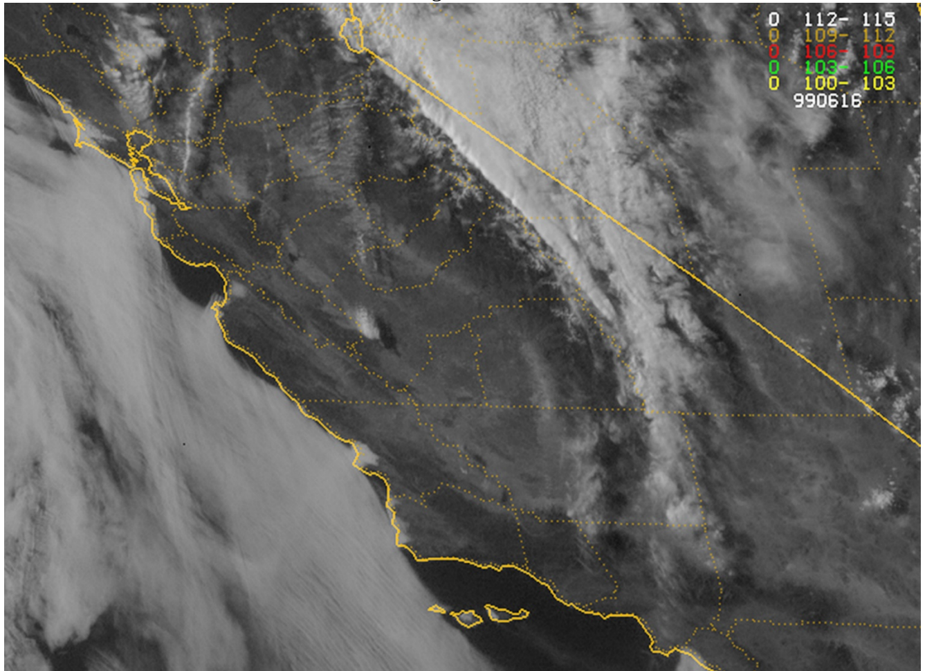
Figure 36: Full Range Sierra Wave
