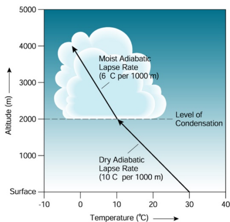
Figure 22: Lapse Rate Change with Condensation
