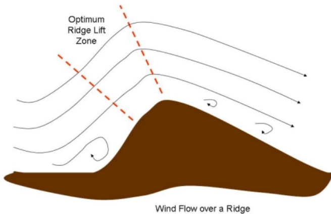
Figure 3: Diagram - Wind Flow over a Ridge and Turbulence
