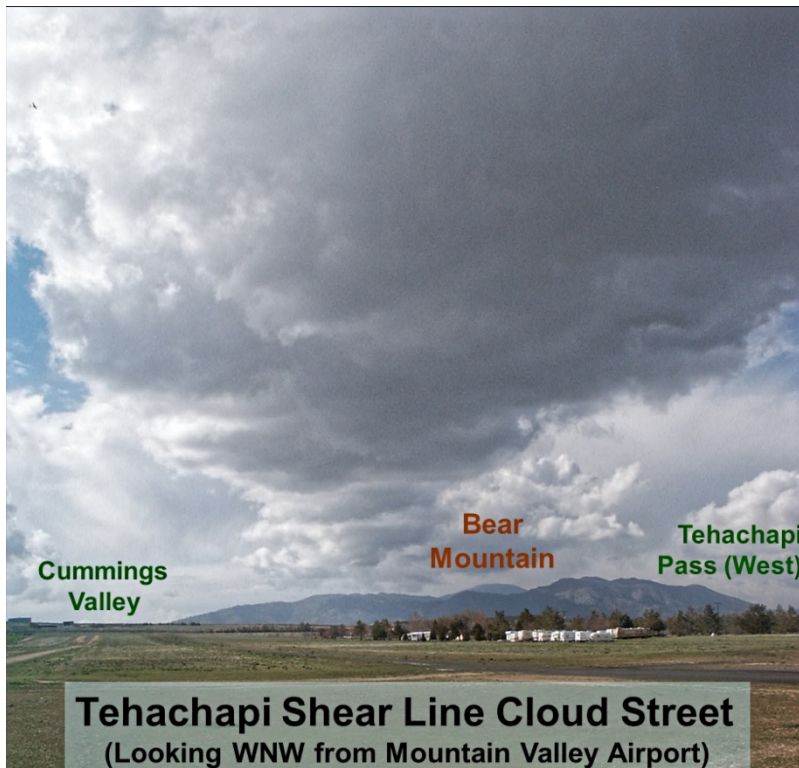
Figure 58: Tehachapi Shear Line Cloud Street
