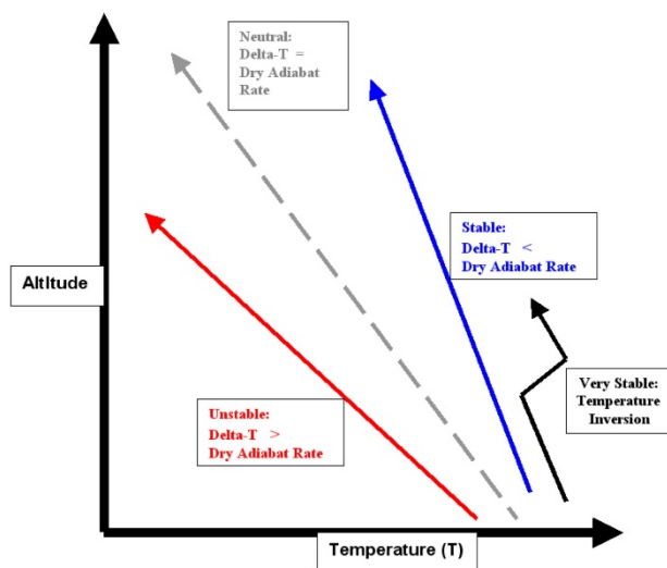
Figure 10: Atmospheric Instability Relative to Lapse Rates
