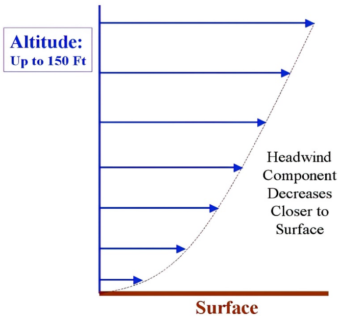
Figure 78: Wind Gradient in the Friction Layer
