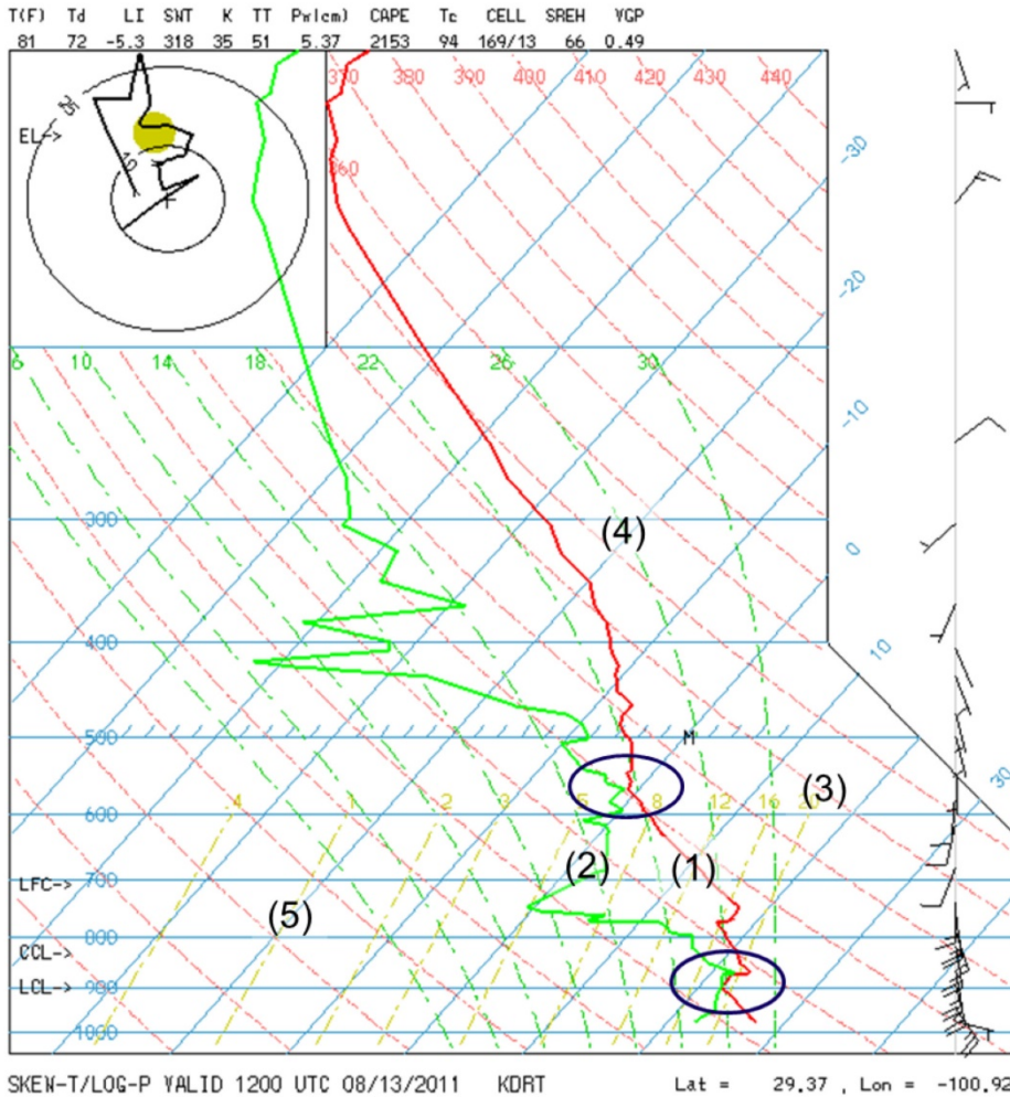
Figure 20: Example Skew-T Energy Diagram
