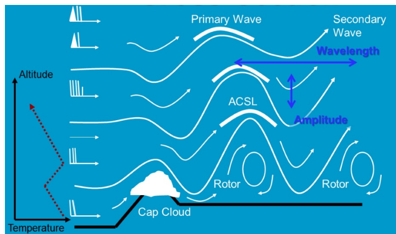
Figure 29: Conceptual Model of Mountain Lee Wave
