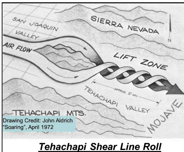
Figure 56: Tehachapi Shear Line Roll
