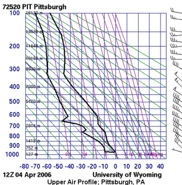
Figure 5: Sounding, Pittsburgh, April 4
