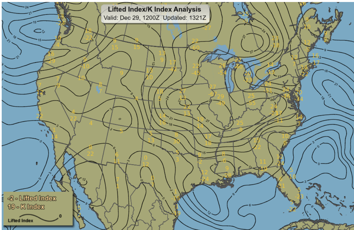
Figure 73: The Lifted Index Analysis Chart
