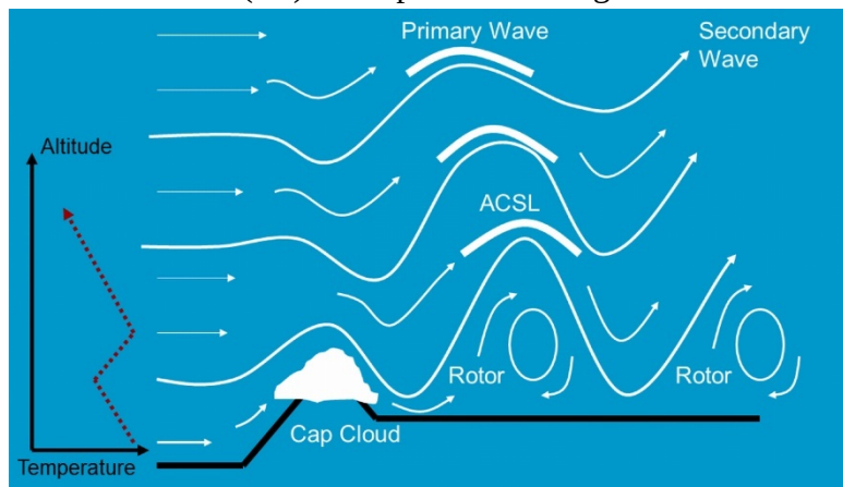
Figure 25: Mountain Lee Wave in Section
