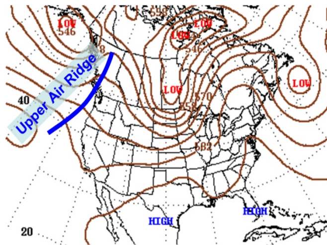
500 Mb Upper Air Chart; June 11, 2012
