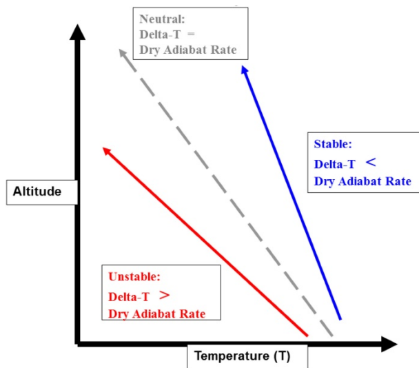
Figure 2: Atmospheric Instability Relative to Lapse Rates
