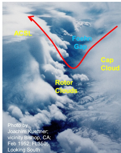
Figure 28: Foehn Gap
